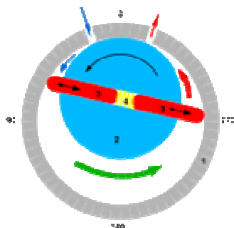
Fixed displacement vane pump
