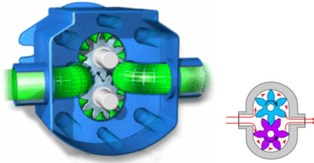
Gear pump with external teet
