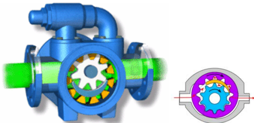
Gearpump with internal teeth
