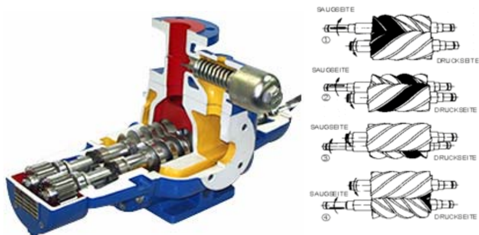
Principle of screw pump
